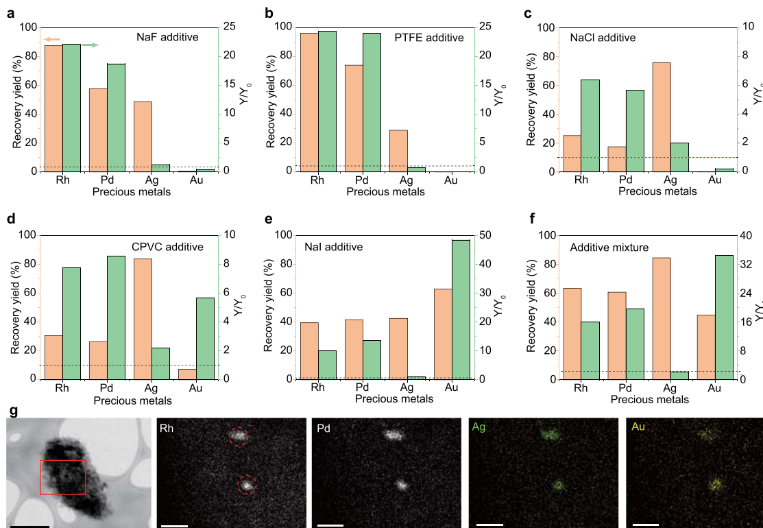
Fig. 2 Halide assisted improvement of recovery yield. Recovery yield of precious metals by using (a) NaF, (b) PTFE, (c) NaCl, (d) CPVC, (e) NaI, and (f) mixture of NaF, NaCl, and NaI, as additives. Y_0 and Y mean the recovery yield of precious metals without and with additives, respectively. The dashed line denotes Y/Y_0 = 1 , meaning that there is no advantage of the additive if Y/Y_0 \leq 1 . The recovery yields were the average of three independent flash Joule heating (FJH) experiments ( n = 3 ). g Scanning transmission electron microscopy (STEM) image of the collected solids, and energy dispersive spectroscopy (EDS) maps of Rh, Pd, Ag, and Au at the rectangular region. Scale bar in STEM image, 0.5 \mu\text{m} ; scale bars in EDS maps, 100 nm. The dashed circles in Rh show the clustered alloys.
