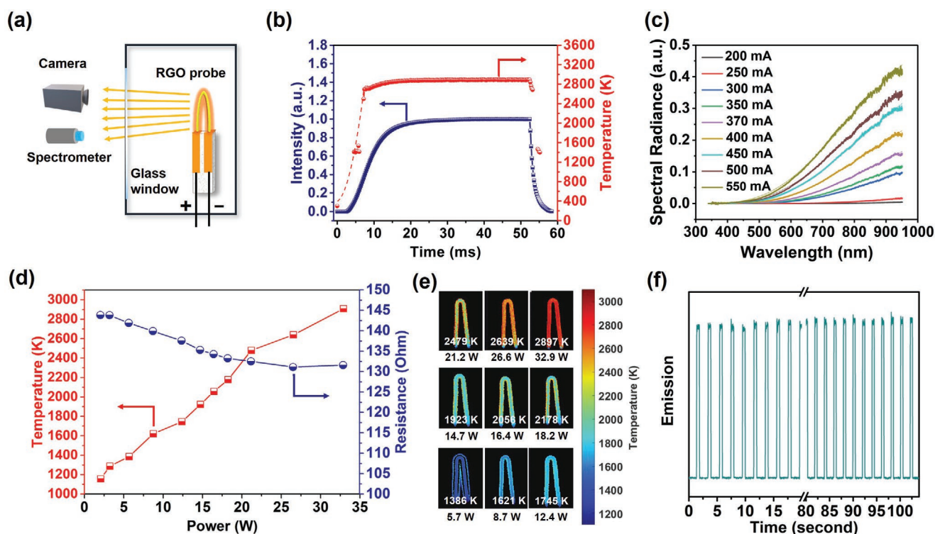
Figure 4. High temperature heating performance of RGO probe under Joule heating. a) Schematic diagram of the operation of RGO probe in the glove-box with argon atmosphere and temperature monitoring by a high-speed camera and spectrometer. b) The temporal evolution of emission and temperature during the rapid Joule-heating process. c) The emission spectra of an RGO probe Joule-heated under different input powers. d) The temperatures of the electrical Joule-heated RGO thermal probe as a function of the input power. e) The images recorded by the high-speed camera of the RGO probe under different input powers. f) The RGO probe can be stably turned on and off without degradation.
