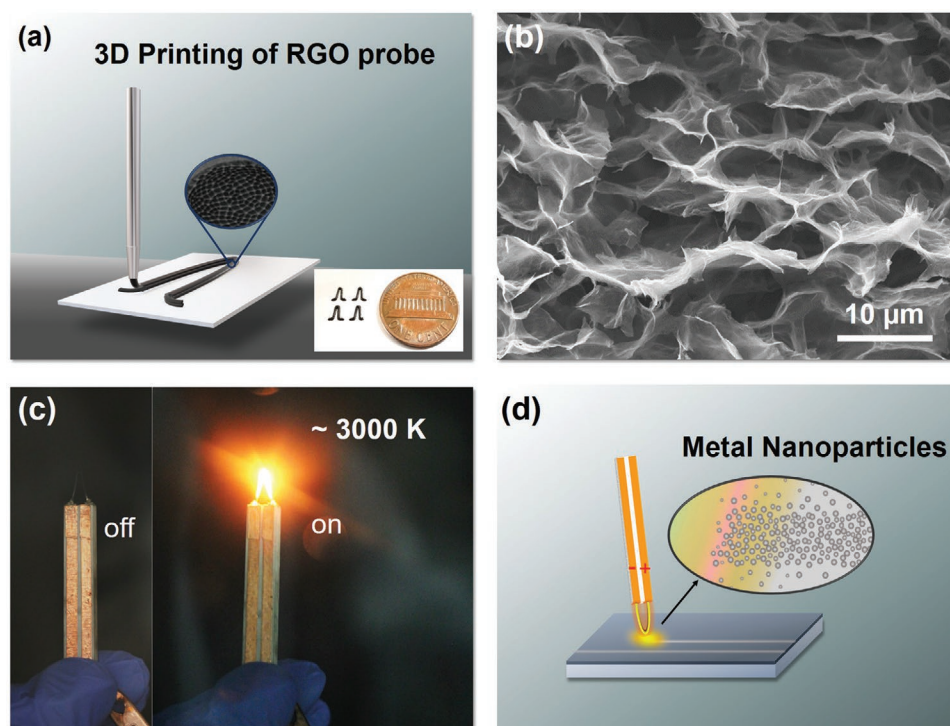
Figure 1. 3D printing of RGO probes. a) Schematic diagrams of 3D printing of RGO probe. Insets: the cellular microstructure of the RGO probe (middle) and arrays of represented as-printed RGO probes (bottom). b) Cross-sectional SEM image of the RGO probe, which shows a cellular microstructure. The cellular microstructure of the RGO probe is expected to experience a high temperature due to larger contact resistance. c) Optical image of the operation of an RGO thermal probe at “off” and “on” states ( \sim 3000 K). The RGO thermal probe device made by fixing the probe on an alumina ceramic handle with copper electrodes. The operation of the thermal probe is performed by supplying a driving current. d) Schematic demonstration of the thermal patterning of metal NPs on the substrate through a rapid radiative heating process by the high-temperature RGO thermal probe.
