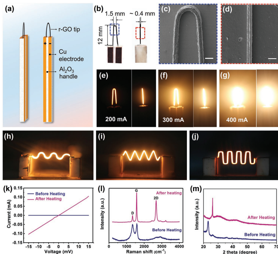
Figure 3. High-temperature RGO thermal probes triggered by electrical Joule heating. a) Schematic diagram of the side (left) and front (right) views of the RGO thermal probe on an alumina ceramic handle attached to copper electrodes. b) Optical images of the front (left) and side (right) views of the RGO thermal probe with a narrow tip width (1.5 mm), a thin filament thickness of \approx 400 \mu\text{m} , and a height of 12 mm. The size and shape of the RGO probe can be easily adjusted by the printing program and nozzle diameter. c,d) The front and side view SEM images of the RGO probe. Scale bar is 500 \mu\text{m} . e–g) Front and side images of the RGO thermal probe under high temperature operations at input currents of 200, 300, and 400 mA, respectively. Optical images of the operation of with h) S-, i) saw-toothed- and j) right-angle-shaped RGO filament feature probes triggered by the applying current of 300 mA. k) The voltage as a function of the driving current for the RGO thermal probe before and after the Joule heating treatment. l) Raman spectra and m) XRD patterns of the RGO thermal probe before and after high-temperature Joule heating treatment.
