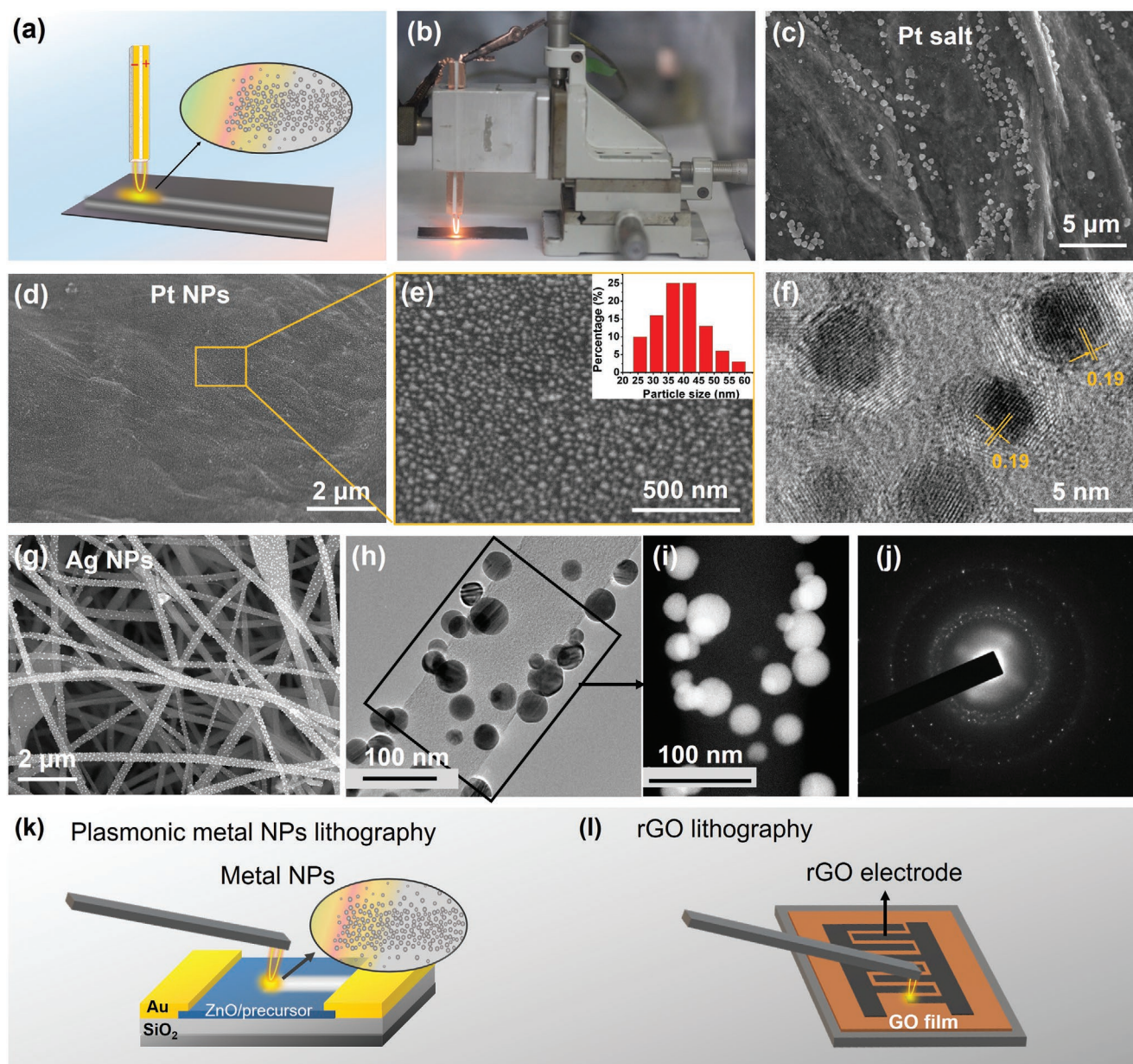
Figure 5. Synthesis of Pt and Ag nanoparticles by the RGO thermal probe. a) Schematic demonstration of the thermal patterning of metal NPs on the surface of a nano-carbon substrate through a rapid radiative heating process by the high-temperature RGO thermal probe. b) Optical image of the setup and its operation for the fabrication of Pt NPs on an RGO film using the high-temperature thermal probe triggered by electrical Joule heating. c) SEM image of the platinum chloride precursor aggregates deposited on the RGO film. d,e) SEM images of Pt NPs on the RGO film after the high-temperature synthesis. Inset is the size distribution histogram of the Pt NPs on the RGO surface. f) The high-resolution TEM image of the Pt NPs indicating the lattice spacing is 0.19 nm, which corresponds to the (200) crystalline plane. g–i) SEM and TEM images of the Ag NPs synthesized on CNFs. j) SAED pattern of the Ag NPs. Scalebar in the inset is 500 nm. k–l) Schematic of RGO probe-based thermal scanning lithography for the fabrication of a plasmon field-effect transistor k), and the selective reduction of GO to interdigitated RGO electrodes l).
