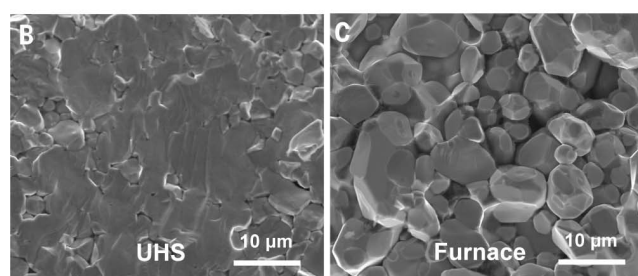
Fig. 2. Rapid sintering of ceramic materials. (A) Typical temperature profile of the UHS process. The whole process takes <1 min. The SEM images demonstrate the reaction process of the LLZTO ceramic over a 10-s isothermal hold of UHS sintering. RT, room temperature. (B and C) Fracture cross-sectional
