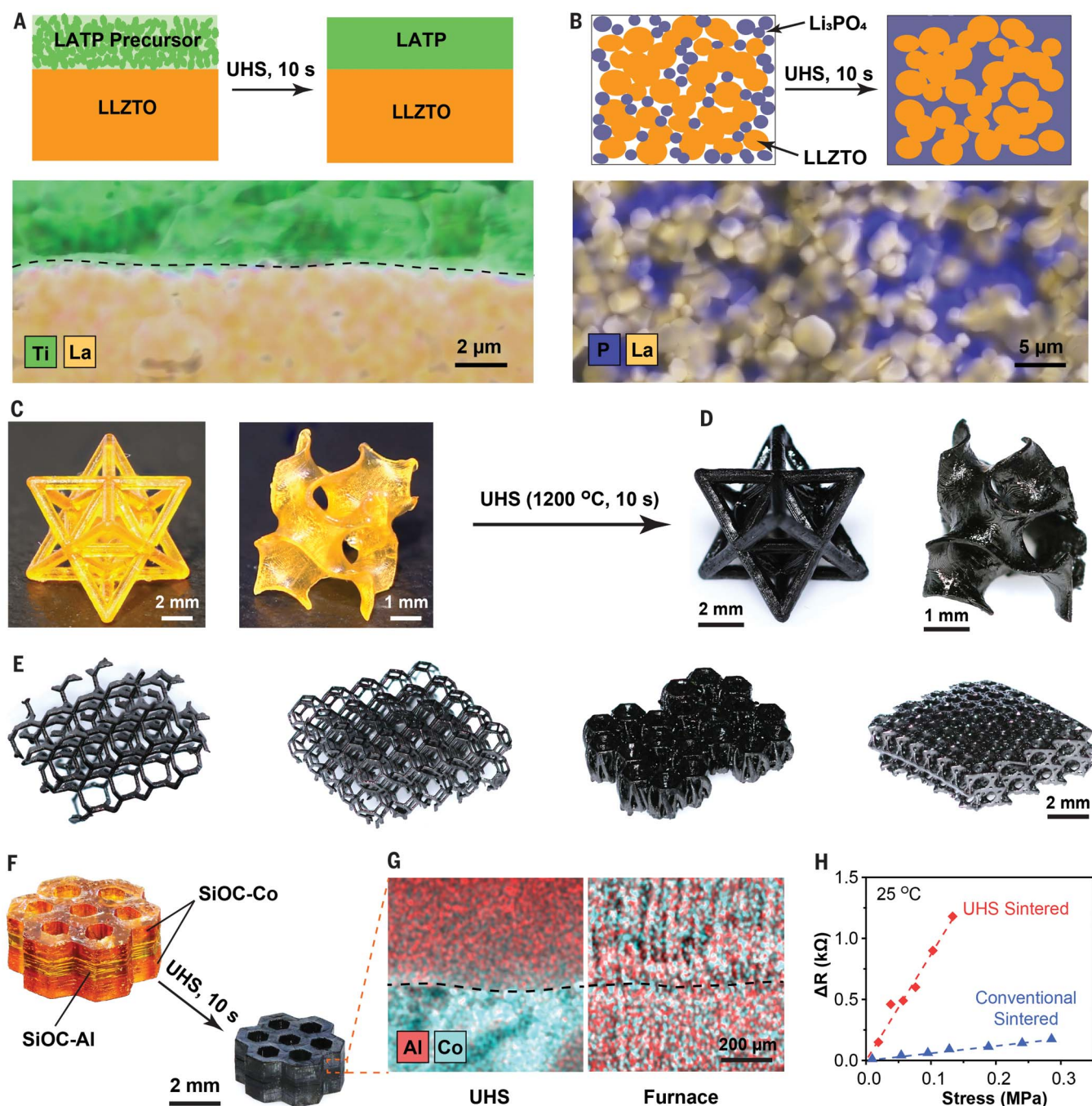
Fig. 4. Structures enabled by the UHS sintering technique. (A and B) Schematics and energy dispersive spectroscopy mapping of the cosintered LATP-LLZTO bilayer SSE (A) and the LLZTO- \text{Li}_3\text{PO}_4 composite SSE (B). (C) Photographs of the SiOC polymer precursor printed as a single material. (D) Photographs of the SiOC samples sintered by the UHS method, showing the uniform material shrinkage and maintained structures. (E) Four UHS-sintered complex structures with different
