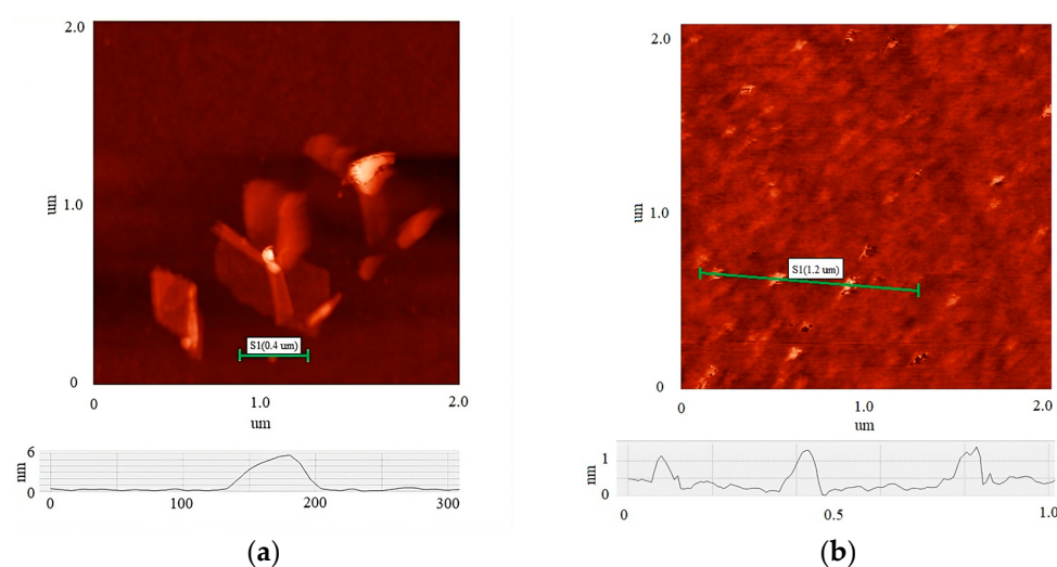
Figure 2. AFM images of individual flakes: (a) MOG; (b) aMOG-200. The height profiles of the flakes are shown at the bottom.
