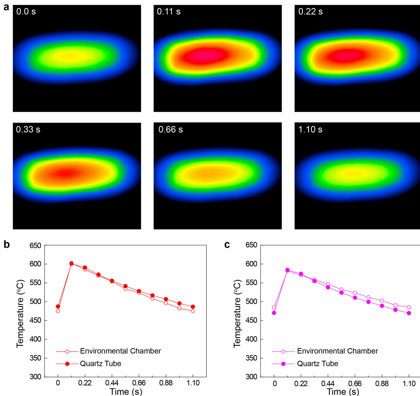
Extended Data Fig. 3 | Temperature measurement using the customized quartz tube with a small opening. a, Temperature maps of the heater and reactor layers at various time points during one heating cycle of 1.10 s (power on time: 0.11 s at about 22 V; power off time: 0.99 s), measured in the customized quartz tube with a small opening (about 7 \times 14 mm) on the tube wall. The temperature scale is the same that as shown in Fig. 2g. This temperature measurement features better accuracy, as the bilayer structure is housed in a quartz tube setup similar to the real STH process but has lower spatial resolution because of the limited size of the opening on the quartz tube
