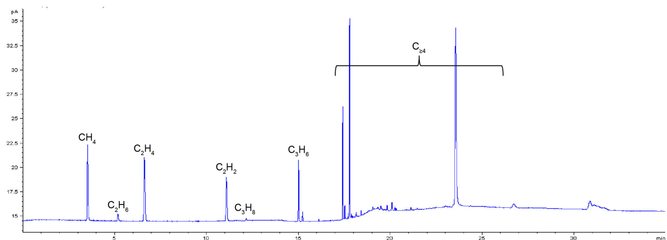
Extended Data Fig. 9 | A typical gas chromatograph by GC-FID of the gaseous products from the STH process with PET using a heating duration of 0.11 s at about 26 V in a period of 1.10 s. Acetylene is observed as one of the gaseous products, which is consistent with the \beta -CH hydrogen-transfer
