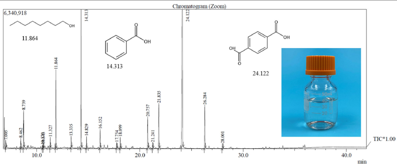
Extended Data Fig. 8 | Gas chromatograph by GC-MS of the liquid products from PET pyrolysis by means of STH using a heating duration of 0.11 s at about 26 V in a period of 1.10 s. Inset, digital image showing the collected products (about 2 wt% in acetone) after three batches of the STH process with
