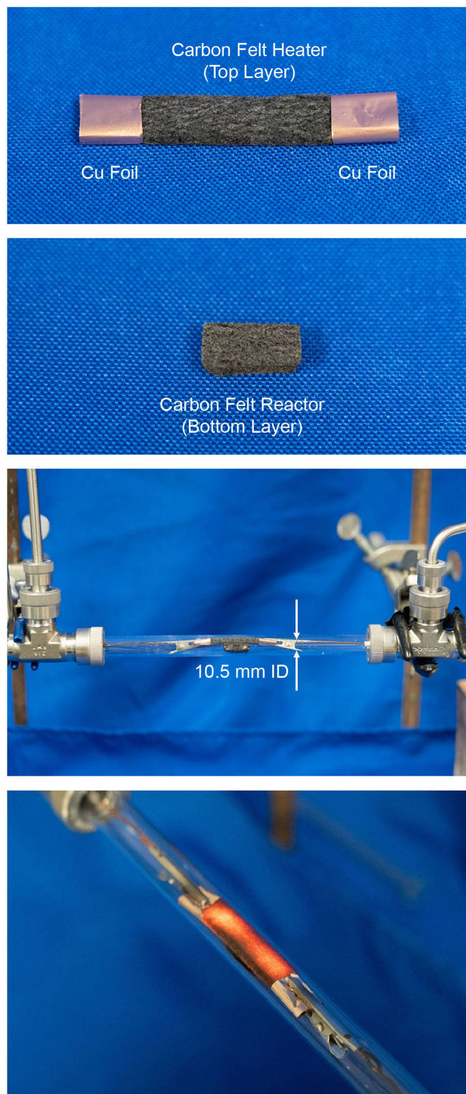
Extended Data Fig. 1 | The assembly of the STH system. A thinner layer of carbon felt (about 2.3 mm) is used as the top heater layer. The two ends of the top heater layer are wrapped with Cu foil electrodes for Joule heating. The top and bottom layers are placed in soft contact (without external pressure) for the STH process. A quartz tube with 10.5 mm inner diameter was used to contain the carbon bilayer structure and the reactant reservoir. The bottom image shows the heater layer exhibiting a bright orange colour as we apply an electrical current through the top heater layer, demonstrating its Joule-heating capabilities.
