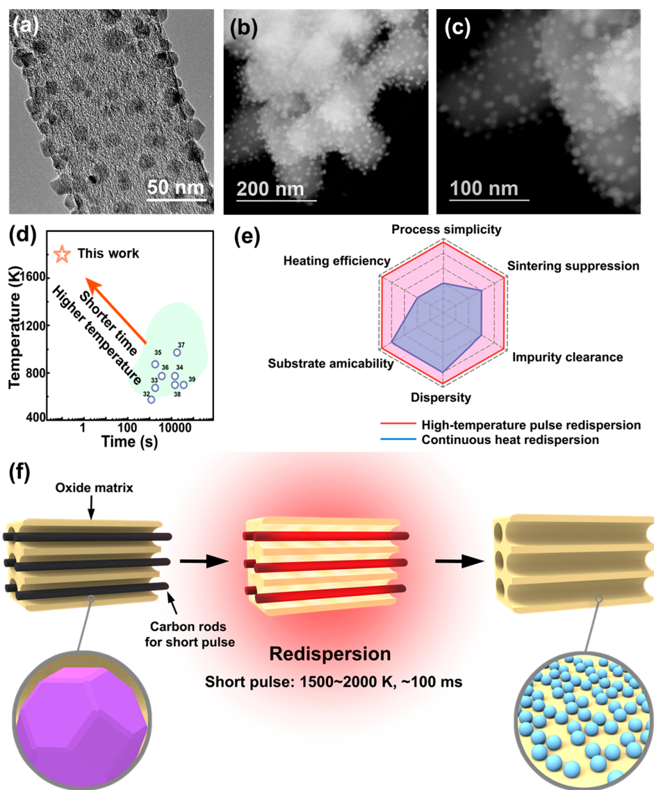
Figure 5. (a) TEM image of Cu nanoparticles redispersed from \text{CuCl}_2 particles. (b) and (c) STEM-HAADF images at different magnifications of Cu nanoparticles redispersed on a porous \text{Al}_2\text{O}_3 substrate. (d) Comparison of the heating time and temperature between this work and previous studies, 32–39 demonstrating the significantly shorter reaction time and higher heating temperature of our technique. (e) A radar plot showing a comparison between high-temperature pulse and continuous heat approaches to nanoparticle redispersion. (f) Schematic for the fast redispersion process of supported nanoparticle catalysts.
