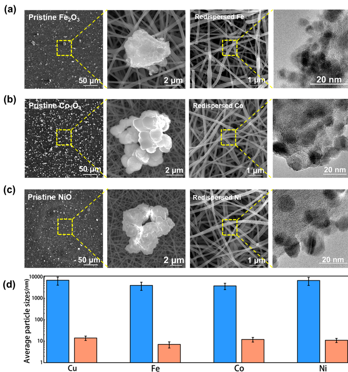
Figure 4. Universality of the high-temperature pulse method for various metal oxide and metal nanoparticles before and after redispersion, respectively, including (a) \text{Fe}_2\text{O}_3 and Fe, (b) \text{Co}_3\text{O}_4 and Co, and (c) NiO and Ni. (d) Statistics of the particle size change before (blue) and after (red) treatment.
