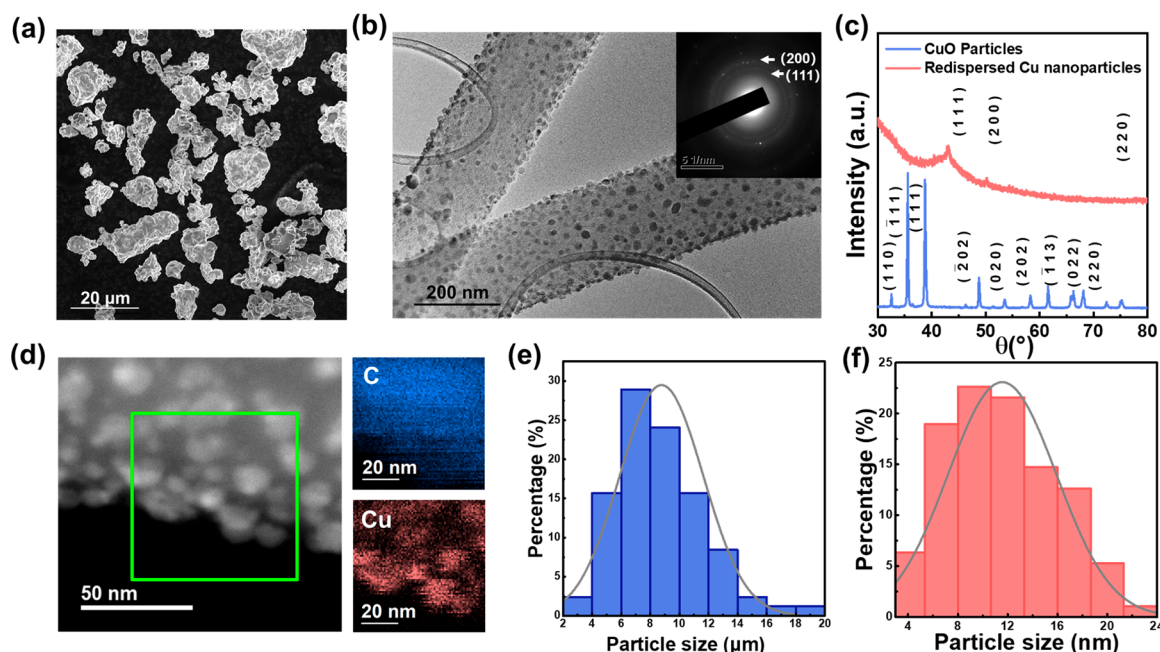
Figure 2. Characterization of Cu nanoparticle redispersion on a CNF substrate after the high-temperature pulse. (a) SEM image of the large CuO particles. (b) TEM image of the redispersed Cu nanoparticles anchored on the CNF substrate. The inset image demonstrates the electron diffraction rings of the Cu nanoparticles. (c) XRD pattern of the Cu nanoparticles confirms the reduced metal after regeneration. (d) EDX mapping of the Cu nanoparticles on the CNF substrate. (e, f) Particle size distribution of the CuO particles (e) before and (f) after redispersion.
