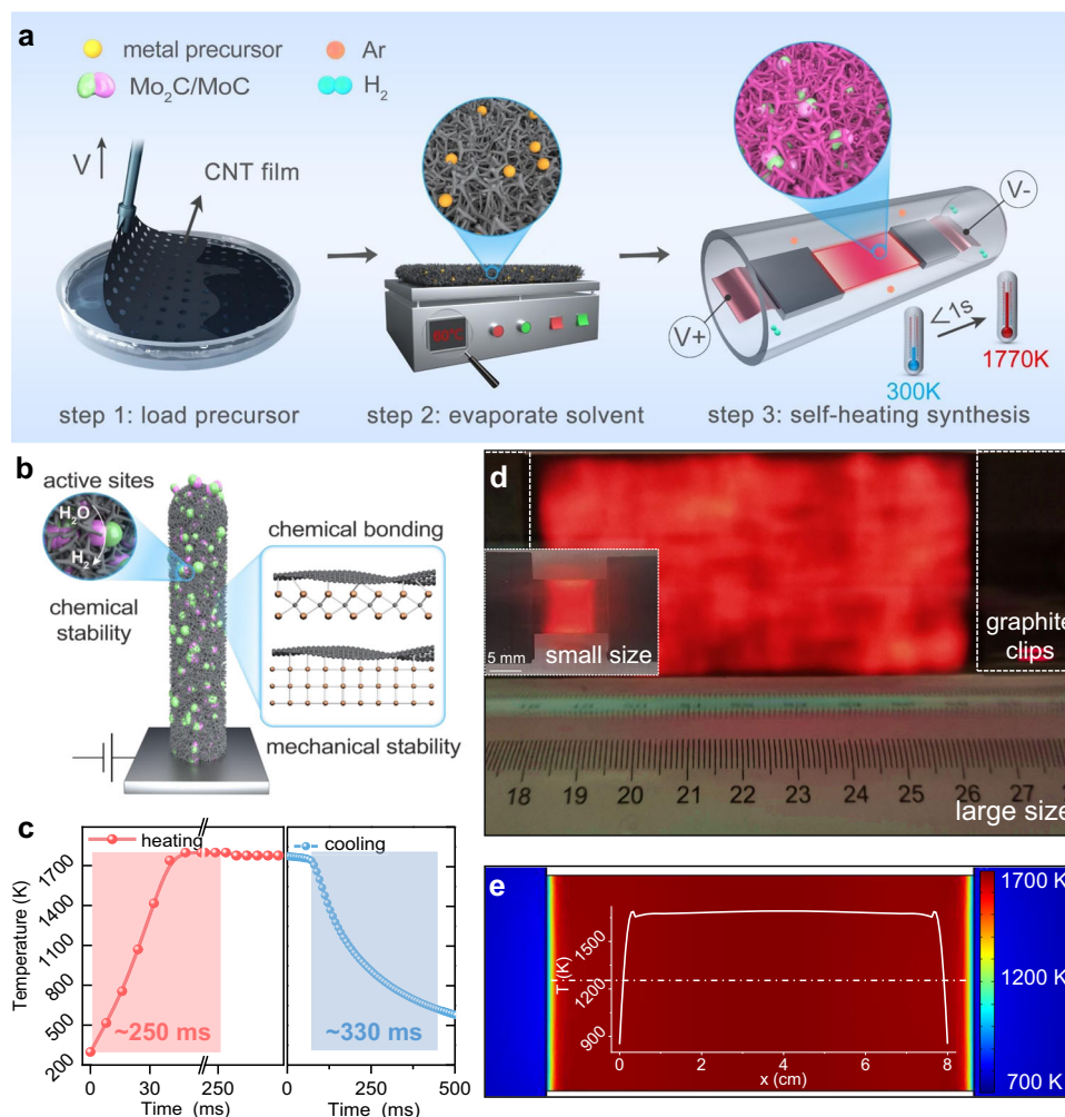
Fig. 1 Ultrafast self-heating synthesis. a Schematic illustration of the synthesis of \text{Mo}_2\text{C}/\text{MoC}/\text{CNT} films by the self-heating method. b \text{Mo}_2\text{C}/\text{MoC}/\text{CNT} film as an HER electrode. c Temperature-Time curve of heating (left) and cooling (right) process during self-heating. d Optical pictures of the CNT film at high temperature in a large size (80 mm \times 40 mm) and a small size (15 mm \times 8 mm, inset). e Simulation of temperature distribution (colour contour) at \sim 1700\text{ K} via COMSOL Multi-Physics software for the large-size film. The top-layer curve shows the temperature distribution along the centerline.
