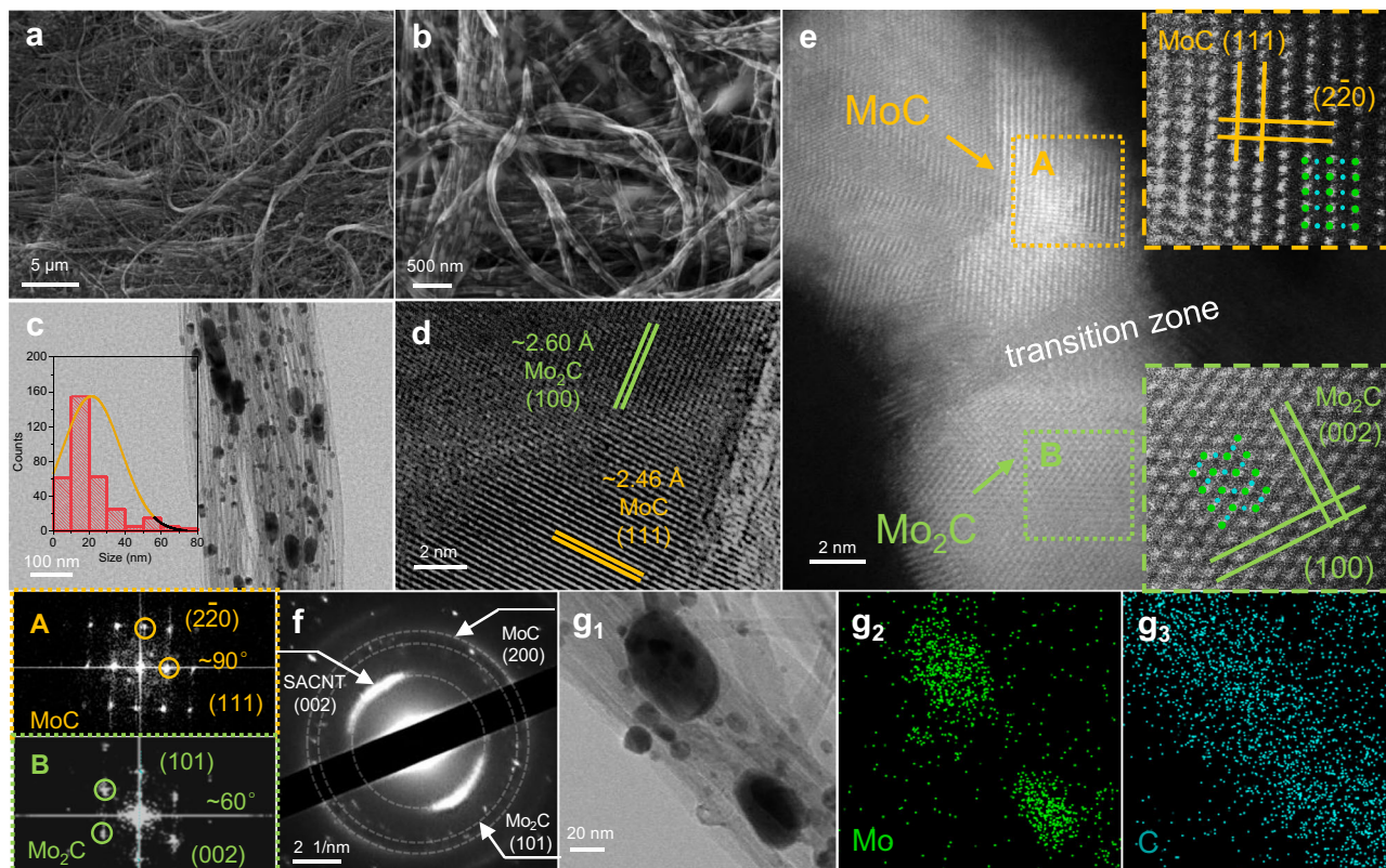
Fig. 3 Electron microscopic characterizations of \text{Mo}_2\text{C}/\text{MoC}/\text{CNT} films. a, b SEM images of \text{Mo}_2\text{C}/\text{MoC}/\text{CNT} film. c TEM images of \text{Mo}_2\text{C}/\text{MoC}/\text{CNT} film. The inset is the statistics of \text{Mo}_2\text{C}/\text{MoC} particle size distribution. d HRTEM images of the interface between \text{Mo}_2\text{C} (100) and \text{MoC} (111) in \text{Mo}_2\text{C}/\text{MoC}/\text{CNT} film. e HAADF-STEM image of \text{Mo}_2\text{C}/\text{MoC} . The inset is HAADF-STEM image of \text{MoC} phase and \text{Mo}_2\text{C} phase, as well as the FT patterns. Green dots represent Mo atoms, and blue dots represent C atoms. f SAED pattern of \text{Mo}_2\text{C}/\text{MoC}/\text{CNT} film. g EDS mapping shows the distribution of Mo and C elements.
