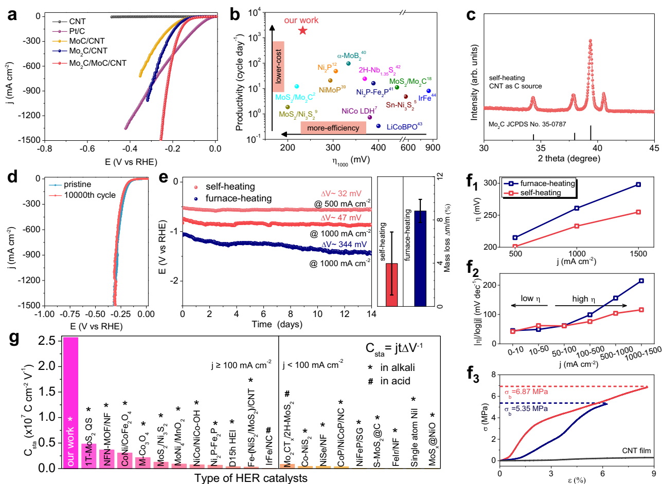
Fig. 4 Electrocatalytic HER performance of Mo 2 C/MoC/CNT films. a Polarization curves of Mo 2 C/MoC/CNT film, Mo 2 C/CNT film, MoC/CNT film, pure CNT film and Pt/C (20 wt% of Pt) in 1 M KOH. b Comparison of overpotentials at 1000 mA cm -2 versus productivity (synthesis cycles in a day) among HER catalysts maintaining activity at high current density. c XRD patterns of self-heating samples only use CNT as carbon sources. d Polarization curves of a pristine Mo 2 C/MoC/CNT film and working after 10000 CV cycles. e Long-term test of self-heating and furnace-heating samples at 500 or 1000 mA cm -2 without iR compensation (left). A mass loss of self-heating and furnace-heating sample after 5 min of ultrasonic treatment in 50 mL alcohol (right). The error bars represent standard deviations. f 1 The overpotential of self-heating and furnace-heating samples at 500, 1000, and 1500 mA cm -2 in 1 M KOH, respectively. f 2 The ratios of \Delta\eta/\Delta\log|j| for self-heating and furnace-heating samples in different current density ranges. f 3 The mechanical tensile curves of self-heating sample, furnace-heating sample, and pure CNT film. g Comparison of long-term stability of various HER catalysts at both small and high current densities.
